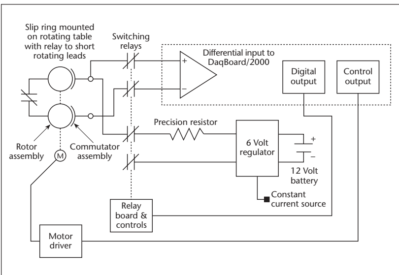
The block functional diagram illustrates the DaqBoard/2000’s ability to both acquire data and provide motor control. Each DaqBoard’s analog input port handles up to 16 slip-ring/commutator measurement channels, one DAC output drives a servomotor on the slip ring assembly, and some of the digital inputs are used for discrete-signal monitoring.
